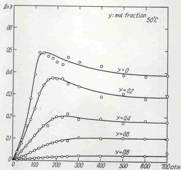
Fig. 5. Activity coefficients of argon in argon-ethylene mixtures.
