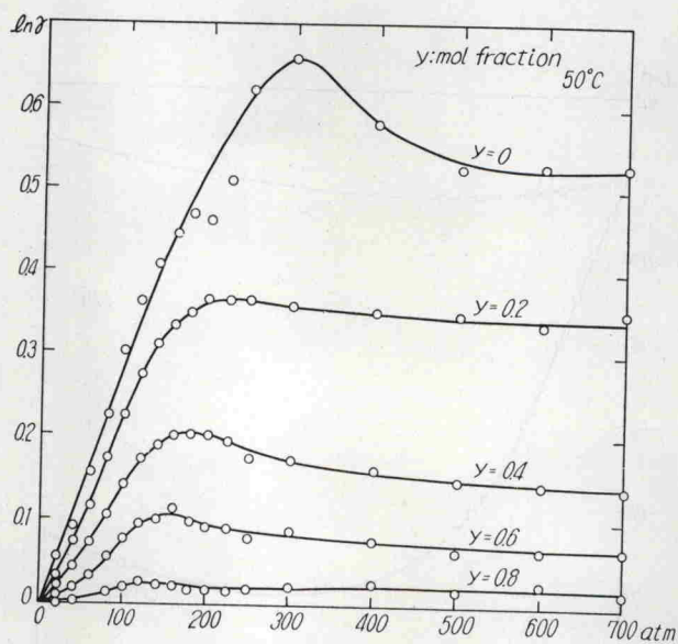
Fig. 6. Activity coefficients of ethylene in argon-ethylene mixtures.
