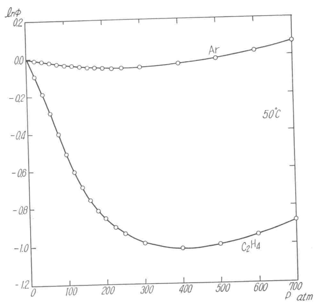
Fig. 4. Fugacity coefficients of argon and ethylene.
