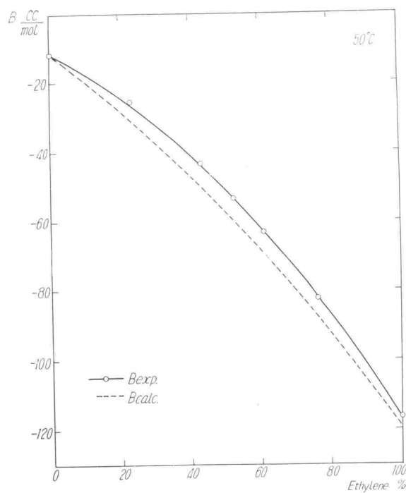
Fig. 3. The 2nd virial coefficients of argon and ethylene mixtures.
